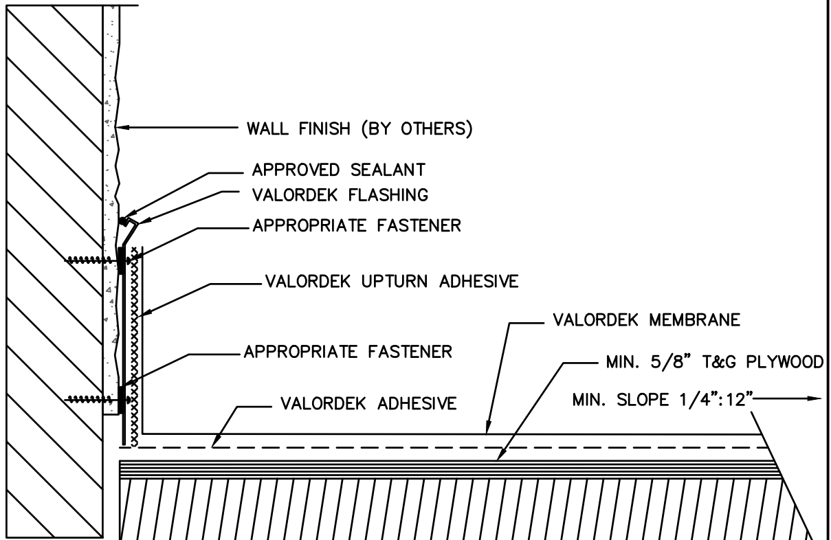
Single Gum Shoe Wall Detail
